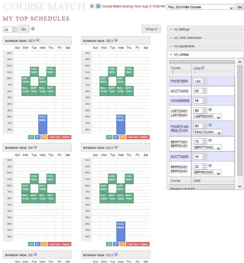
Figure 3. (Color online) A student's top schedules are generated from his or her reported preferences and shown in a separate step before the input is saved
