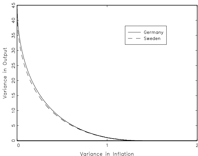
Figure 9: Implied Output-Inflation Variability Frontiers
