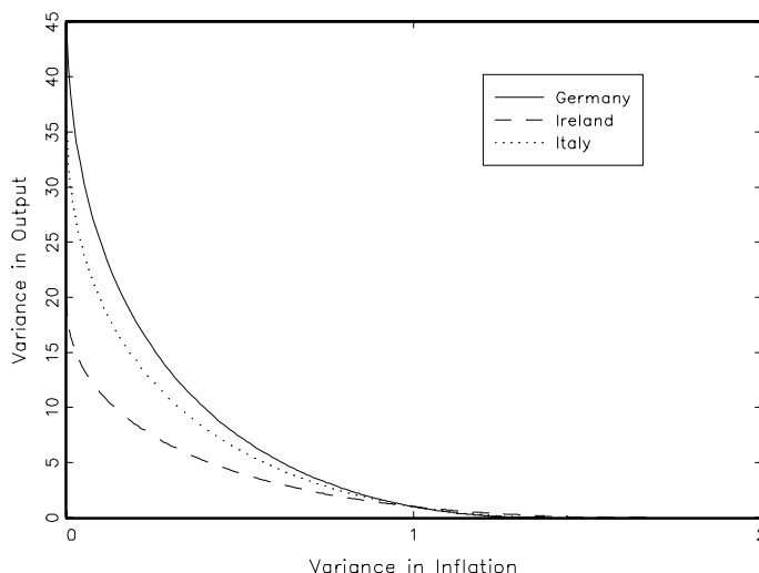
Figure 10: Implied Output-Inflation Variability Frontiers
