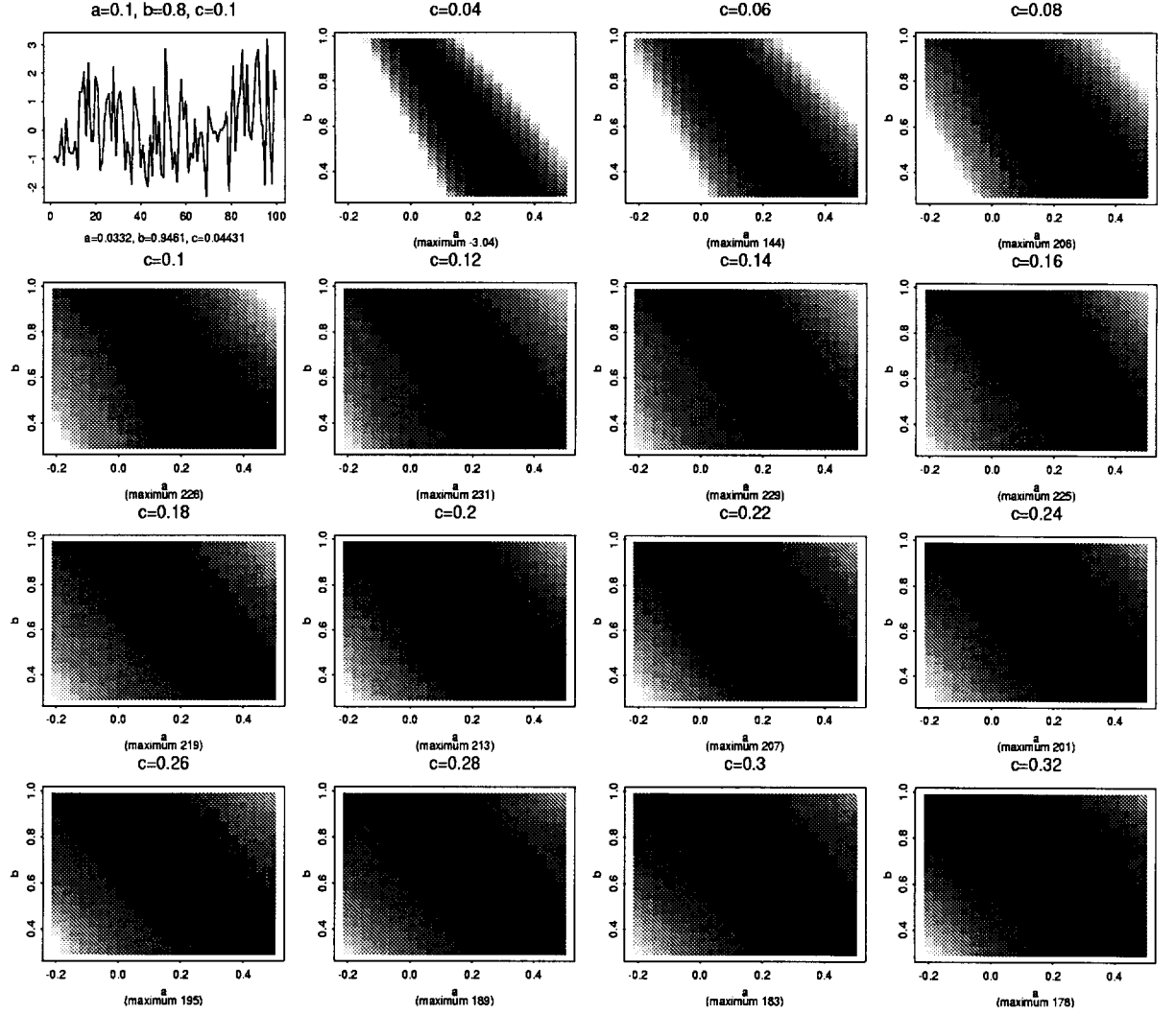
Figure 5: Evaluated slices in c of the log-likelihood ratio associated with (35) for a simulated sample of size T = 100 and 5000 iterations of the completion step. See Table 10 for the parameter values.
