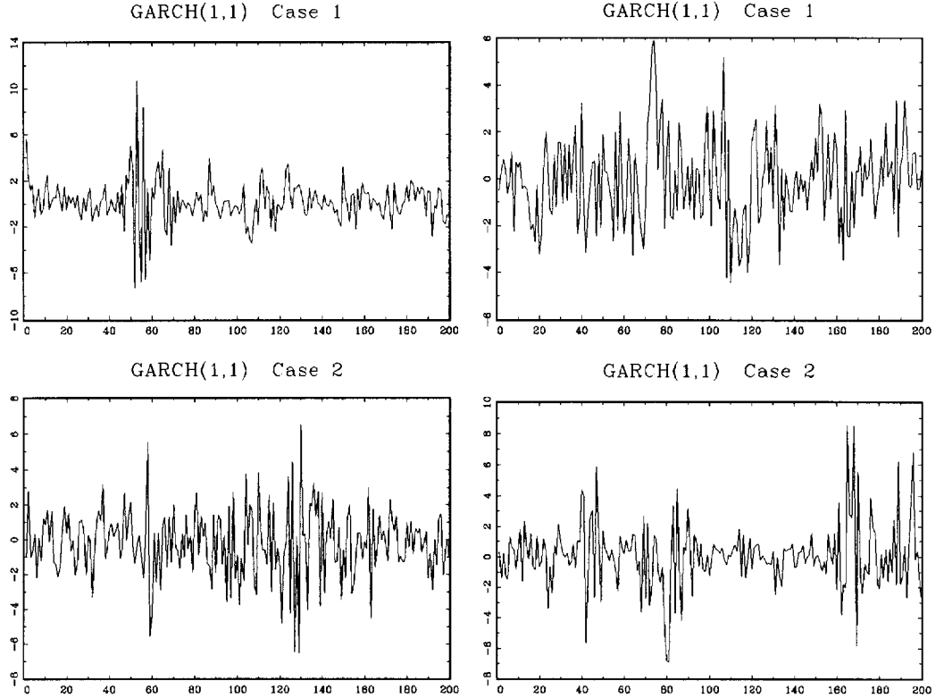
Figure 2: Simulated samples from the GARCH(1,1) model (40), case 1 and 2.
