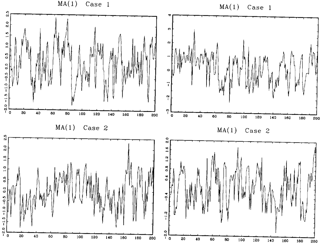
Figure 1: Simulated samples from the MA(1) model (38), case 1 and 2.
