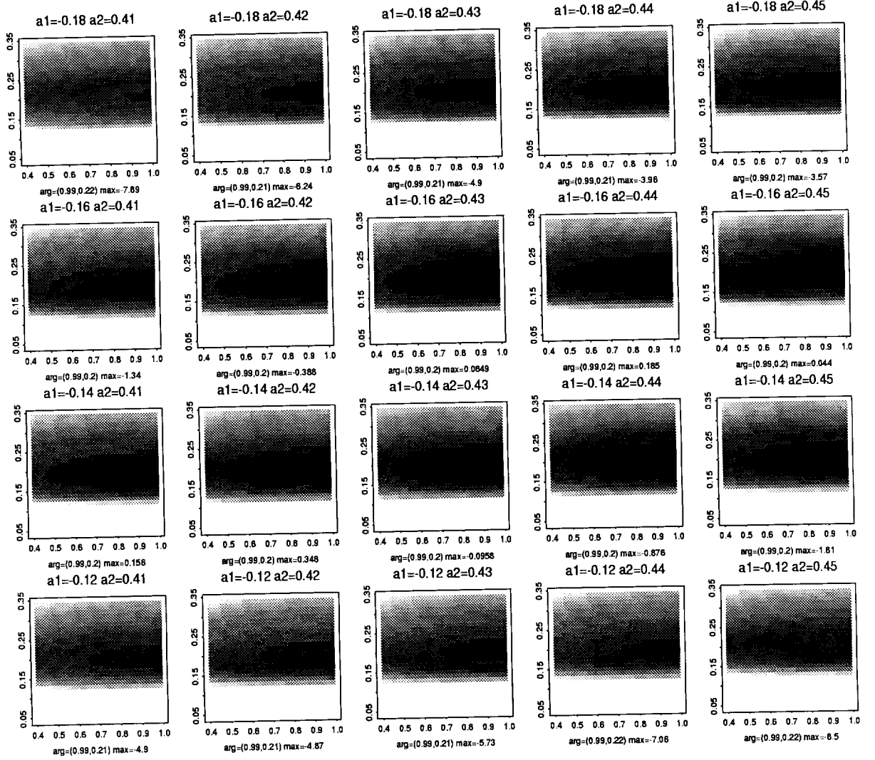
Figure 4: Estimated slices of the log-likelihood ratio for the factor ARCH model (43) for a simulated sample of size T = 100 and 50,000 iterations of the completion step, with a batch size of 50. See Table 9 for the parameter values.
