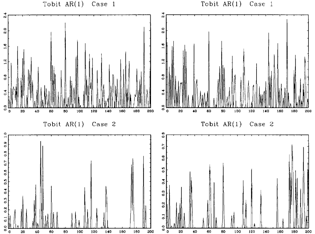
Figure 3: Simulated samples from the Tobit AR(1) model (41), case 1 and 2.
