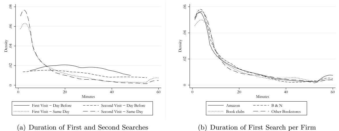
Figure 6: Duration Searches
