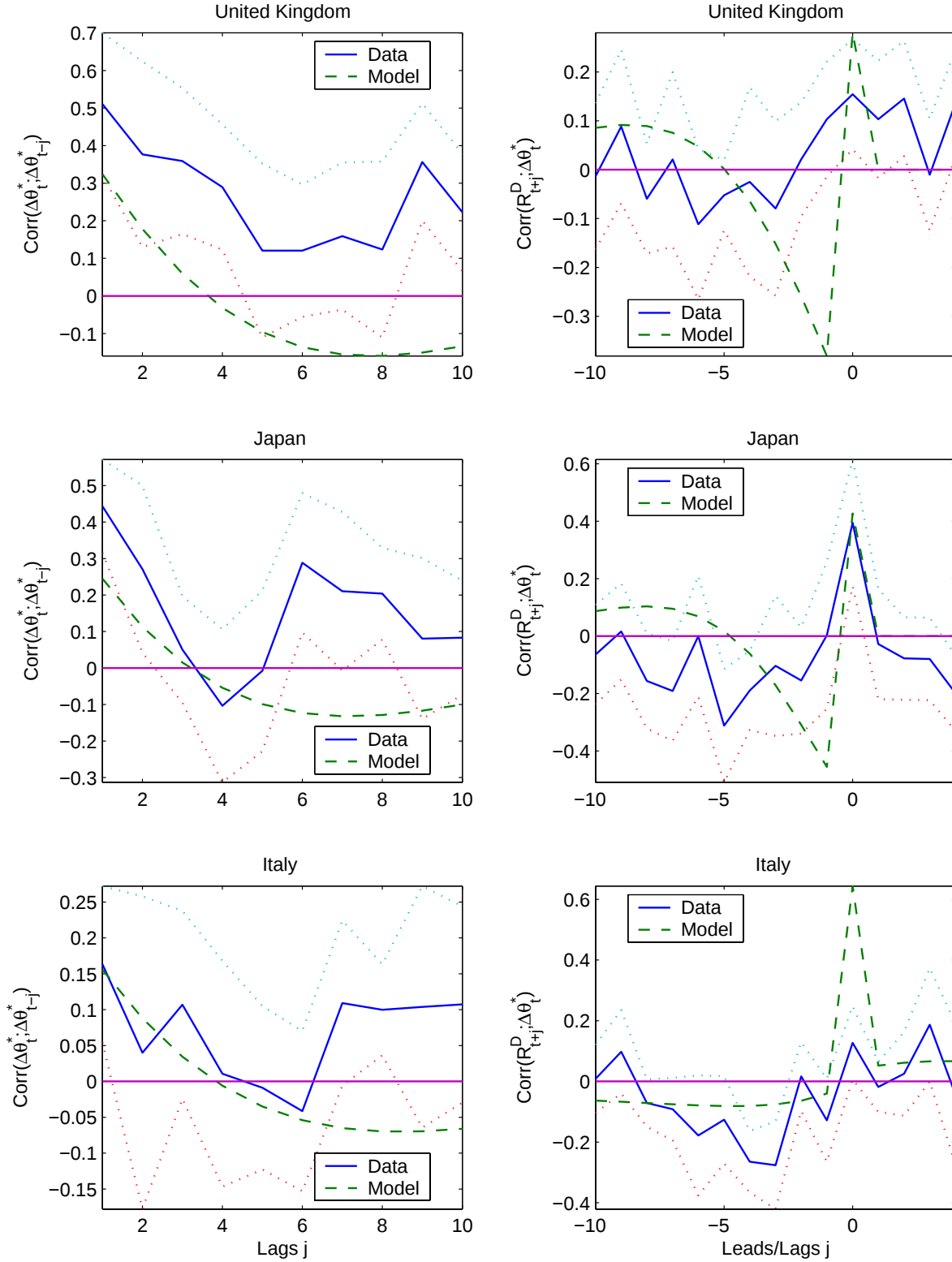
Figure 4: Autocorrelogram of flows and cross-correlogram of returns and flows: U.K., Japan and Italy. Notes: \Delta\theta_t^* is net-purchases of the local asset by US investors; R_t^D is the current return on the local asset. Dotted lines are 90 percent confidence bands.
