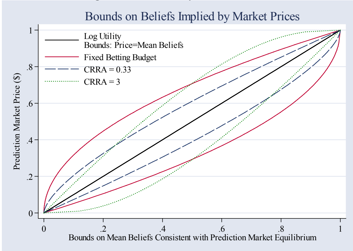
Figure A1: Bounds Analysis in Four Models
