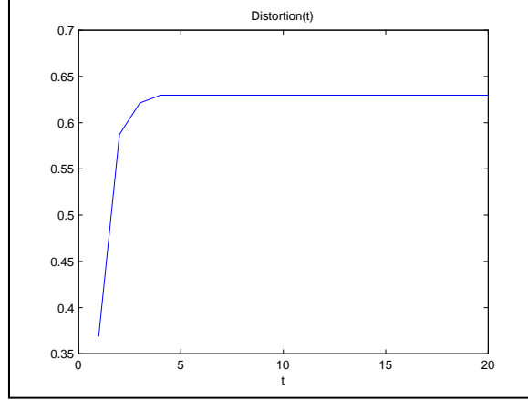
Figure 6: Theorem 3 part 3. Time path of distortions with \beta = 0.5 and \delta = 0.4 .
