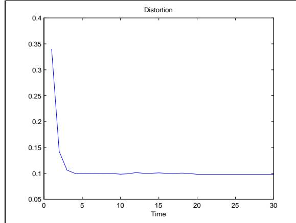
Figure 8: Theorem 4, part 3, almost constant types. The time path of distortions with \beta = 0.8 and \delta = 0.6 .
