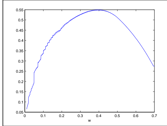
Figure 4: Theorem 3 part 3. Value function with \beta = 0.5 and \delta = 0.4 .
