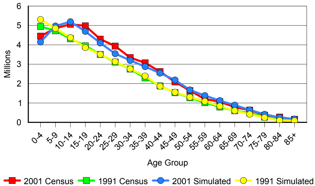
Figure 7.4: Censuses & Simulations
